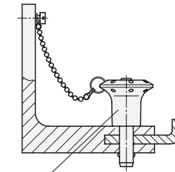
Locking pins Ball lock pins
