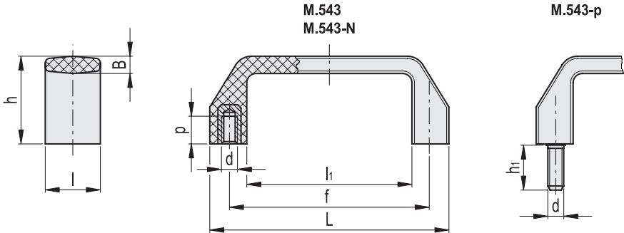
ELESA Original design
